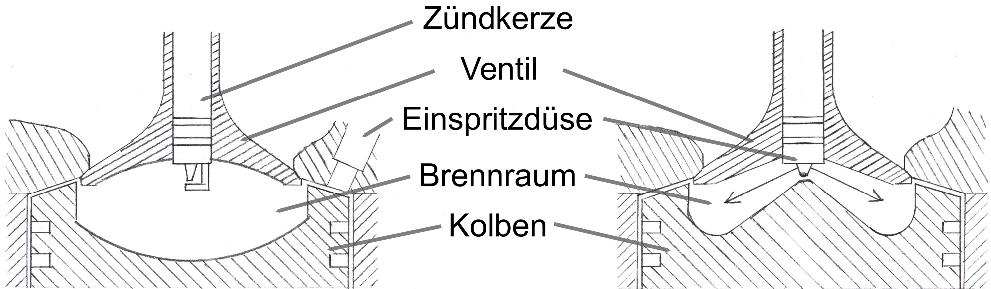
Ottomotor
